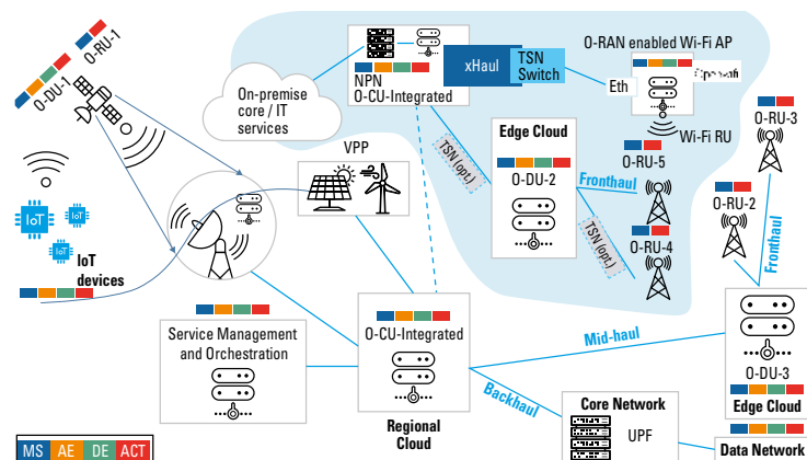
UNITY-6G architecture
